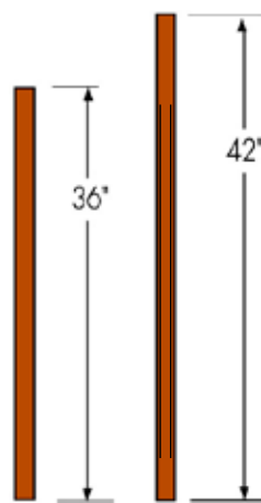
1 3/4" Square 36" and 42" Blank and Chamfer Balusters
