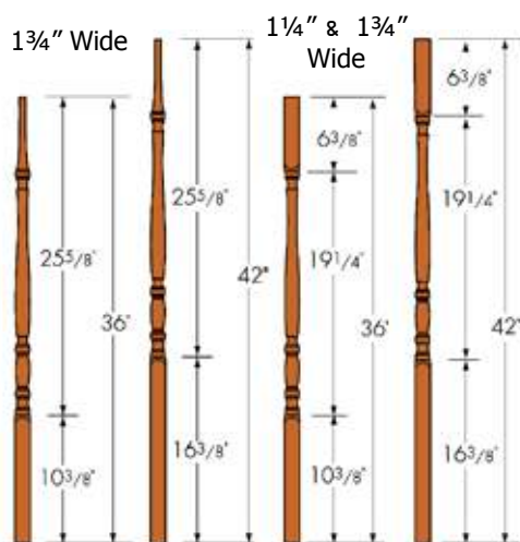
36" and 42" Dowel and Square Top Balusters
