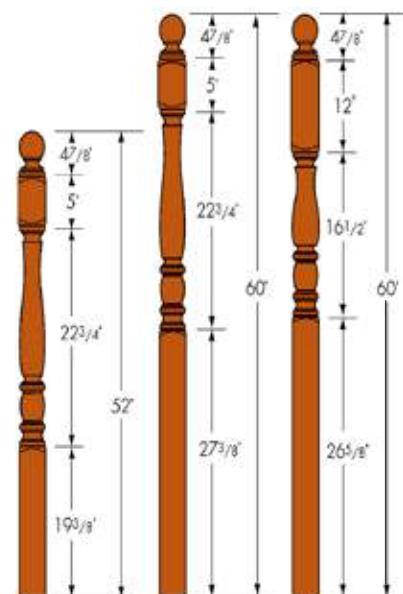
52" Newel 60" Newel Long Face Newel
