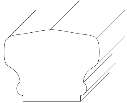
102 - 1 2 3/4" (W) x 2 1/8" (H) (1 5/8" bottom)
