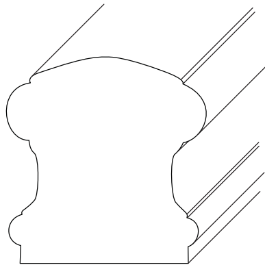
103 - 1 2 3/4" (W) x 2 3/4" (H) (2 1/4" bottom)
