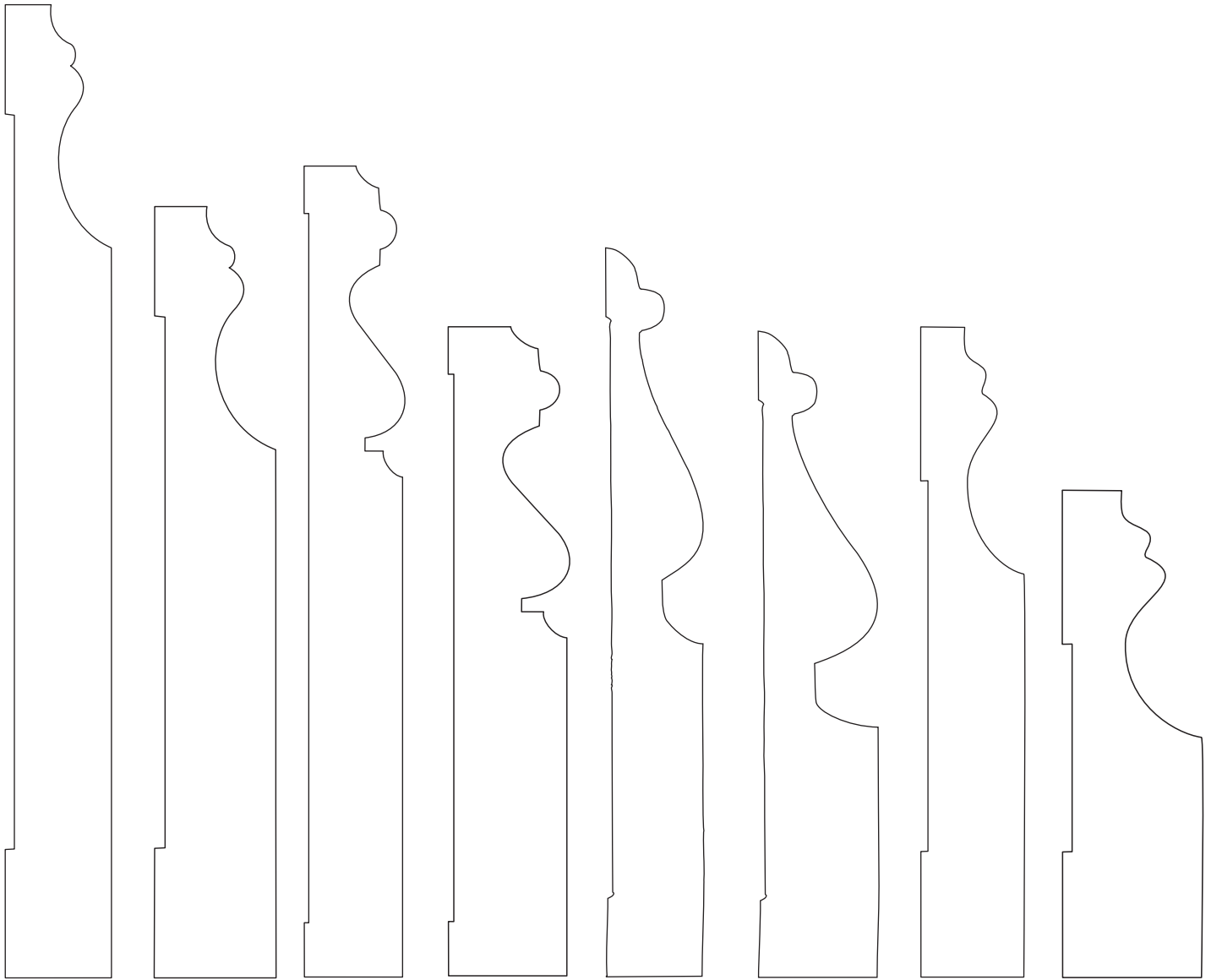
B 5 C 5 B 6 C 6 B 7 C 7 B 8 C 8 5/8" x 6" 3/4" x 4 3/4" 5/8" x 5" 3/4" x 4" 5/8" x 4 1/2" 3/4" x 4 1/2" 5/8" x 4" 3/4" x 3"
