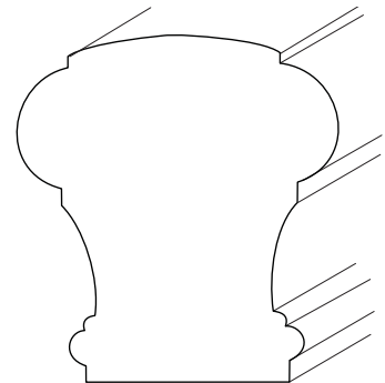
104 - 1 2 3/4" (W) x 2 3/4" (H)
